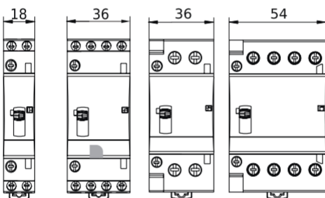
Ex9CH16/20/25M
