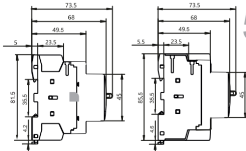
Ex9CH16/20/25M
